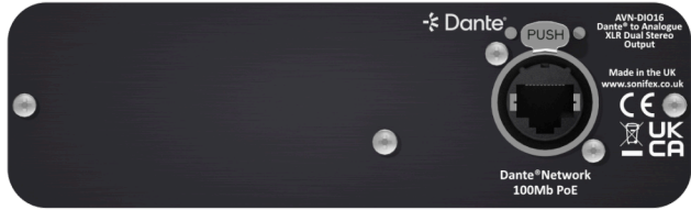
Fig 1: AVN-DIO16 Front Panel
