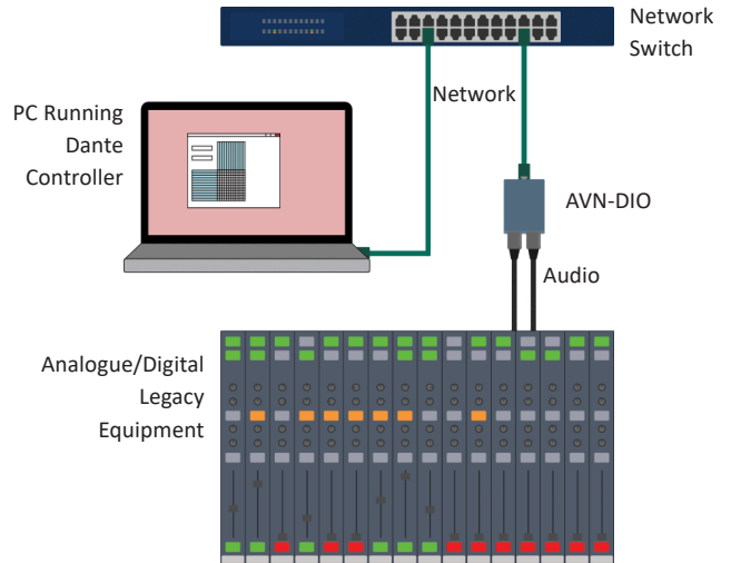
Fig 2: Typical AVN-DIO setup
